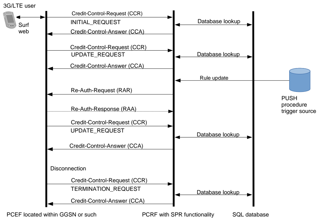
Figure 2 depicts Gx request flow with both PULL and PUSH procedure. SPR functionality is based on SQL backend for example purposes.
