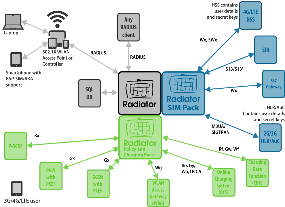
Figure 1. Diameter authentication, policy and charging interfaces supported by Radiator
