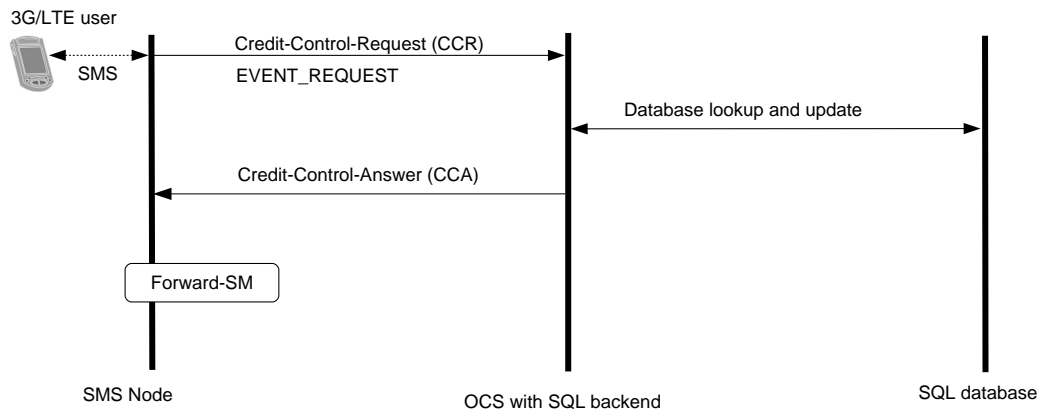
Figure 4. Event based online charging with Direct Debiting
