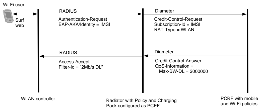
Figure 3. Radiator Policy Configuration Enforcement Function example
